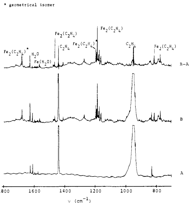
Figure 1. A. Infrared spectrum of matrix-isolated ethylene in argon. Molar ratio of ethylene to argon \approx 5:1000. B. Infrared spectrum of matrix-isolated iron/ethylene in argon. Molar ratio of \text{Fe}:\text{C}_2\text{H}_4:\text{Ar} \approx 15:5:1000. Period of deposition = 30 min. Absorbance of strongest product peak = 0.08. Resolution = 1 cm -1 .
