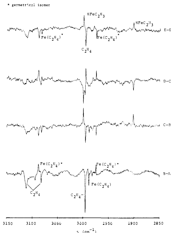
Figure 3. A reversible photolysis study. FTIR difference spectra of the carbon-hydrogen stretching region of Fe/C 2 H 4 in Ar: A, no photolysis; B, λ > 400 nm, 20 min; C, 280 nm < λ < 360 nm, 10 min; D, λ > 400 nm, 20 min; E, 280 nm < λ < 360 nm, 10 min.
