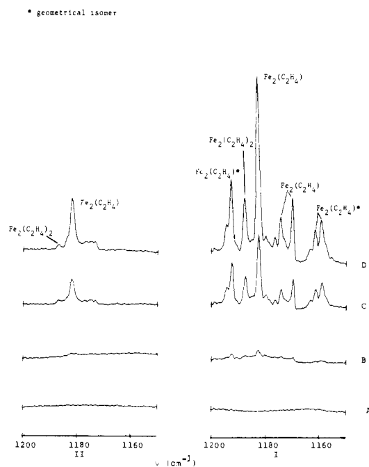
Figure 9. An iron concentration study. The \delta(CH_2) symmetric deformation region of iron/ethylene \pi -complexes. Molar ratio of C_2H_4:Ar(1) or Kr(II) \approx 5:1000 . Molar ratio of Fe:1000Ar ; A = 0, B = 0.8, C = 5.0, and D = 15.0.
