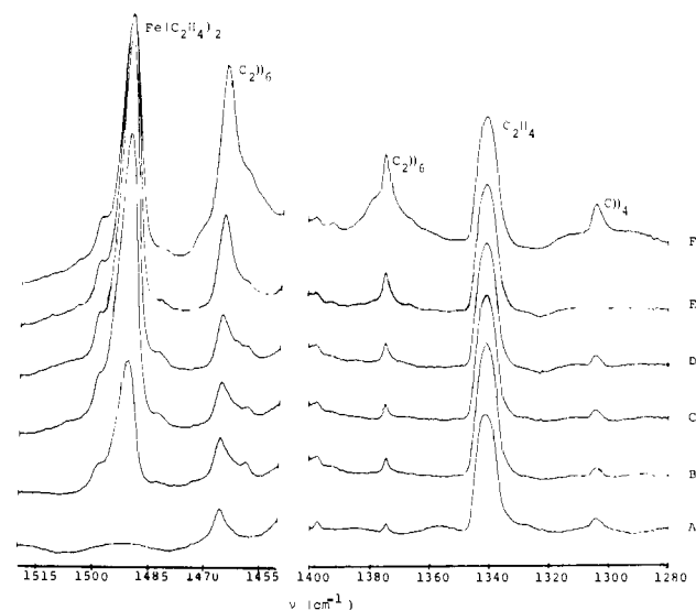
Figure 8. Time dependent photolysis study. The \nu(C=C) stretching and the \delta(CH_2) symmetric deformation regions of iron/ethylene \pi -complexes. Molar ratio of Fe:C_2H_4:Ar \approx 6:124:1000 : A, no iron; B, no photolysis; C, \lambda \geq 400 nm, 20 min; D, 280 < \lambda < 360 nm, 30 min; E, 280 < \lambda < 360 nm, 4 h; F, 280 < \lambda < 360 nm, 16 h.
