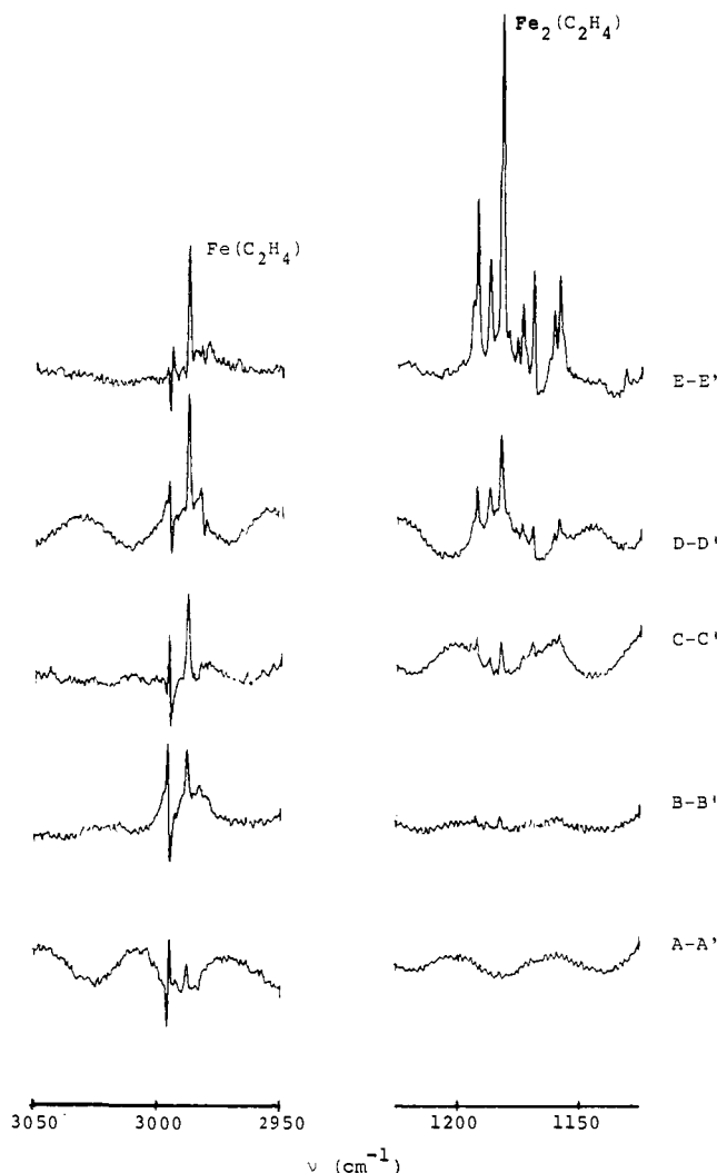
Figure 2. An iron concentration study. FTIR difference spectra of Fe/C 2 H 4 and C 2 H 4 in Ar. Molar ratios for (Fe:C 2 H 4 :Ar): A, 0.2:6.8:1000; B, 0.4:7.0:1000; C, 1.1:6.9:1000; D, 2.2:7.9:1000; E, 7.7:4.9:1000. Molar ratios for (C 2 H 4 :Ar): A', 6.8:1000; B', 7.0:1000; C', 6.9:1000; D', 7.9:1000; E', 4.9:1000.
