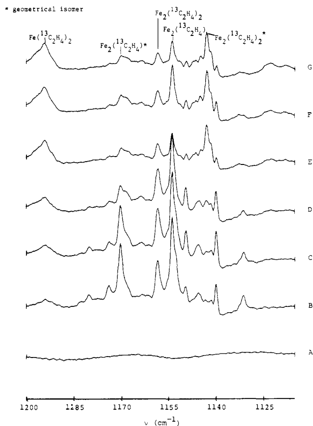
Figure 11. A reversible photolysis study. The \delta(\text{CH}_2) symmetric deformation region of iron/ethylene \pi -complexes. Molar ratio of \text{Fe}:^{13}\text{C}_2\text{H}_4:\text{Ar} \approx 4:8:1000 ; A, no iron; B, no photolysis; C, \lambda \geq 500 nm, 20 min; D, \lambda \geq 400 nm, 20 min; E and G, 280 < \lambda < 360 nm, 30 min; F, \lambda \geq 400 nm, 12 min.
