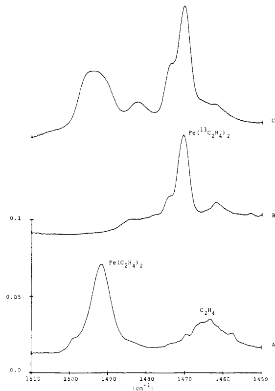
Figure 7. A mixed C_2H_4/^{13}C_2H_4 isotopic study. The \nu(C=C) stretching region of iron/ethylene \pi -complexes. Molar ratio of Fe:C_2H_4:Ar \approx 9.5:52:1000 : A, iron with C_2H_4 in argon; B, iron with ^{13}C_2H_4 in argon; C, iron with C_2H_4/^{13}C_2H_4 in argon.
